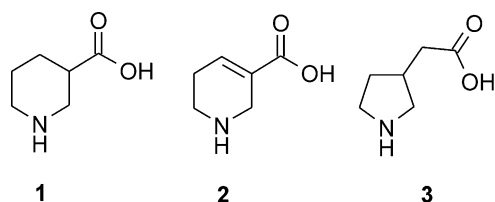
Figure 1. Three cyclic amino acids which act as GABA uptake inhibitors, nipecotic acid 1 , guvacine 2 and homo-β-proline 3 .
