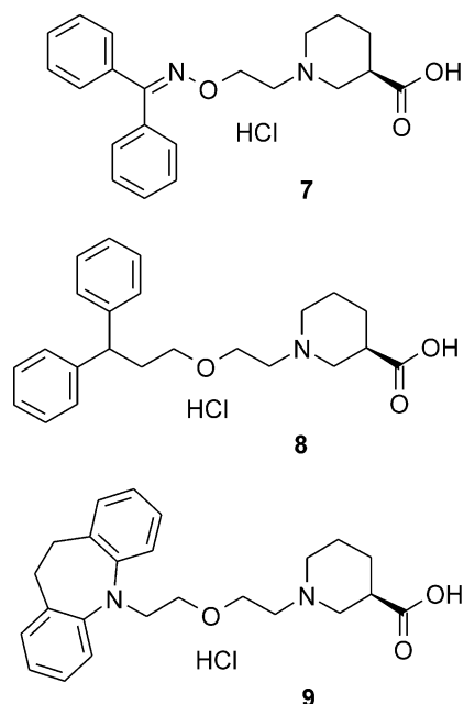
Figure 3. Potent GABA uptake inhibitors with an electronegative moiety introduced in the chain.
