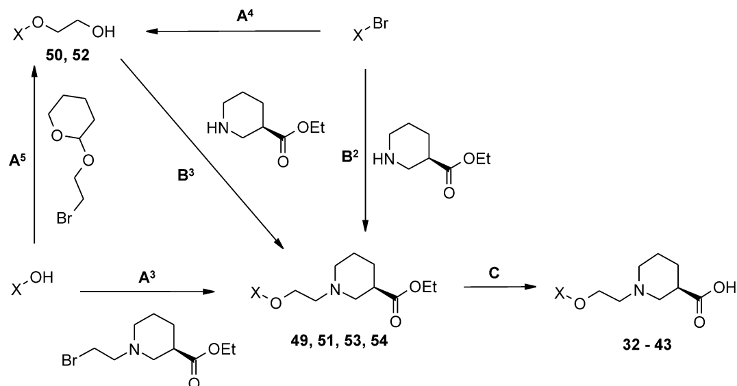
Scheme 2. Synthesis of ether derivatives 32–43. For definition of X, see Table 1. Method A 3 : NaH, toluene or THF, rt; method A 4 : n -BuLi, ethylene glycol, rt. Method A 5 : DMSO, KOH, 100 °C; method B 2 : K 2 CO 3 , MIBK, reflux; method B 3 : (1) TEA, Et 2 O, MsCl, reflux or n -BuLi, THF, MsCl, reflux; method C: (1) NaOH, EtOH, rt; (2) HCl.
