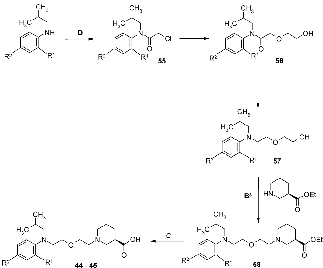
Scheme 3. Synthesis of anilinoalkylethers 44–45. R 1 and R 2 , see Table 1. Method D: (1) (ClCH 2 CO) 2 O, H 2 O, 70 °C; (2) ethylene glycol, DMF, KO 2 Bu, rt; (3) LiAlH 4 , toluene, THF, rt; method B 3 : (1) TEA, CH 2 Cl 2 , MsCl, –10 to 0 °C; (2) Li 2 CO 3 , isopropyl acetate, reflux, method C: (1) NaOH, EtOH, rt; (2) HCl.
