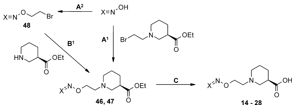
Scheme 1. Synthesis of oxime-ether derivatives 14–28 . For definition of X, see Table 1. Method A 1 : (1) K_2CO_3 , acetone, rt; method A 2 : K_2CO_3 , acetone, BrCH_2CH_2Br , reflux; method B 1 : K_2CO_3 , acetone, reflux; method C: (1) NaOH, EtOH, rt; (2) HCl.
