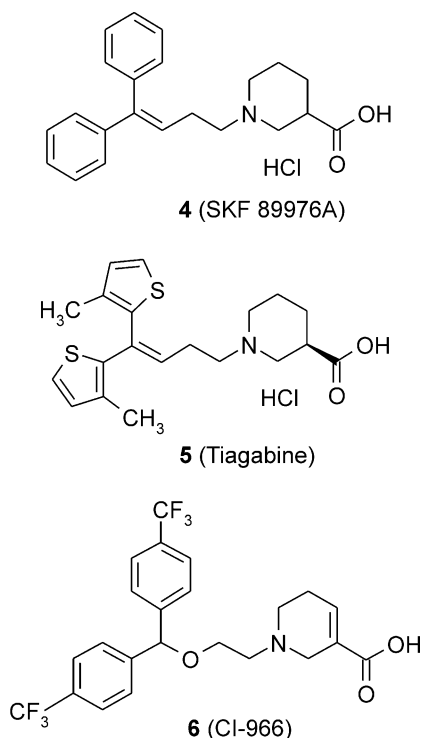
Figure 2. Lipophilic reference GABA uptake inhibitors.
