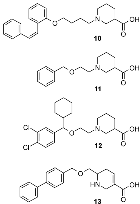
Figure 4. Various known derivatives of nipecotic acid ( 1 ) and guvacine ( 2 ) which does not possess any significant affinity for the GABA uptake site.
